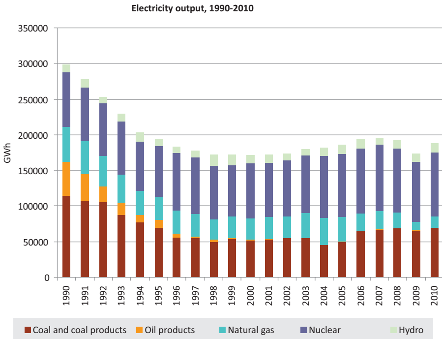
Figure 7 Electricity output 1990–2010
